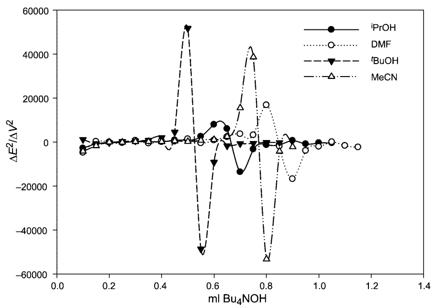
Fig. 4. \Delta E^2/\Delta V^2 vs. ml \text{Bu}_4\text{NOH} Potentiometric titration curves of 0.001M solutions of compound 3d titrated with 0.05M \text{Bu}_4\text{NOH} at 25°
