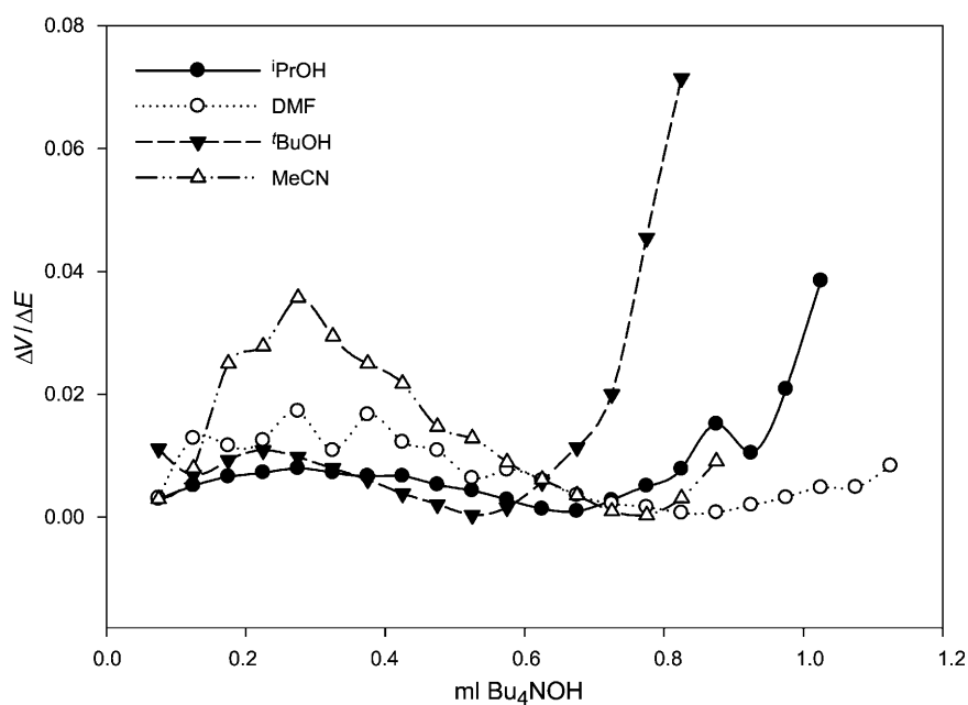
Fig. 5. \Delta V/\Delta E vs. ml \text{Bu}_4\text{NOH} Potentiometric titration curves of 0.001M solutions of compound 3d titrated with 0.05M \text{Bu}_4\text{NOH} at 25°
