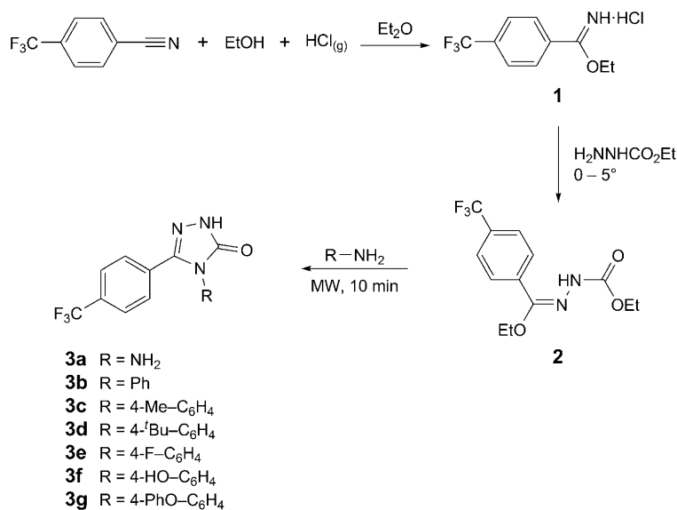
Scheme. Pathway for the Formation of the 3H-1,2,4-Triazol-3-ones
