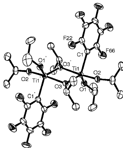
Figure 1. Molecular structure of 1 , showing 50% probability ellipsoids and partial atom-labeling scheme. Hydrogen atoms are omitted for clarity. \text{Ti}(1)\text{--C}(1) 2.1763(17), \text{Ti}(1)\text{--O}(1) 1.7651(13), \text{Ti}(1)\text{--O}(2) 1.7583(12), \text{Ti}(1)\text{--O}(3) 1.9420 (11), \text{Ti}1\text{--O}3' 2.0873(11), \text{Ti}(1) \cdots \text{Ti}(1') 3.2299(6), \text{O}3\text{--Ti}1\text{--O}3' 73.53(5), \text{Ti}1\text{--O}3\text{--Ti}1' 106.47(5), \text{O}(2)\text{--Ti}(1)\text{--O}(1) 101.98(6), \text{O}(2)\text{--Ti}(1)\text{--O}(3) 99.93(5), \text{O}(1)\text{--Ti}(1)\text{--O}(3) 118.89(5), \text{O}(2)\text{--Ti}(1)\text{--O}(3') 167.35(6), \text{O}(1)\text{--Ti}(1)\text{--O}(3') 90.68(5), \text{O}(3)\text{--Ti}(1)\text{--O}(3') 73.49(5), \text{O}(2)\text{--Ti}(1)\text{--C}(1) 91.27(6), \text{O}(1)\text{--Ti}(1)\text{--C}(1) 108.61(7), \text{O}(3)\text{--Ti}(1)\text{--C}(1) 127.13(6).
