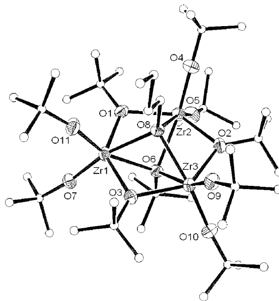
Figure 3. Molecular structure of the cationic part of 3 (the anion [B(C_6F_5)_4]^- and the solvent of crystallization (1/2 CH_3CN ) are omitted for clarity), showing 50% probability ellipsoids and partial atom-labeling scheme. Hydrogen atoms are omitted for clarity. O(1)–Zr(2) 2.179(3), O(1)–Zr(1) 2.192(3), O(2)–Zr(2) 2.169(3), O(2)–Zr(3) 2.175(3), O(3)–Zr(1) 2.184(3), O(3)–Zr(3) 2.192(3), O(4)–Zr(2) 1.921(3), O(5)–Zr(2) 1.918(3), O(6)–Zr(2) 2.324(3), O(6)–Zr(1) 2.334(3), O(6)–Zr(3) 2.352(3), O(7)–Zr(1) 1.922(3), O(8)–Zr(1) 2.276(3), O(8)–Zr(3) 2.310(3), O(8)–Zr(2) 2.339(3), O(9)–Zr(3) 1.921(3), O(10)–Zr(3) 1.924(3), O(11)–Zr(1) 1.914(3), Zr(1)···Zr(3) 3.4083(6), Zr(1)···Zr(2) 3.4087(7), Zr(2)···Zr(3) 3.4079(6), O(11)–Zr(1)–O(7) 99.24(13), Zr(2)–O(1)–Zr(1) 102.49(12), Zr(2)–O(6)–Zr(3) 93.58(10), Zr(1)–O(6)–Zr(3) 93.33(10), Zr(1)–O(8)–Zr(3) 95.99(10), Zr(1)–O(8)–Zr(2) 95.21(10), O(11)–Zr(1)–O(1) 99.65(12).
