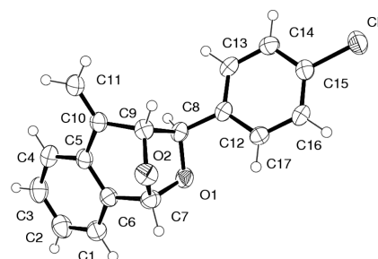
Figure 4. ORTEP representation of (1 R ,9 R ,10 R )- 6j .
