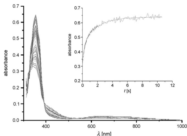
Figure 9. Spectral changes during reaction of I with dioxygen in methanol ( T = -60.1^\circ\text{C} , [\text{complex}] = 0.1\text{ mM} , [\text{O}_2] = 4.25\text{ mM} , t = 10.605\text{ s} ). Inset: Absorbance versus time trace at 353 nm and fit to the sum of two exponentials ( k_{\text{obs}}^1 = (3.1 \pm 0.2) , k_{\text{obs}}^2 = (0.41 \pm 0.03)\text{ s}^{-1} ).
