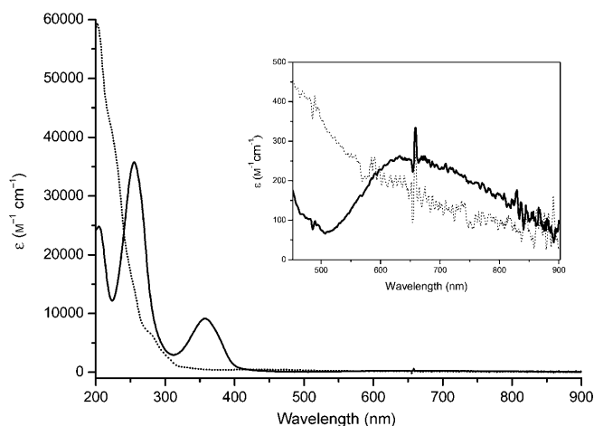
Figure 3. UV/Vis spectra of Ib (dotted line, 8 \times 10^{-5} \text{ mol L}^{-1} ) and II (solid line, 11 \times 10^{-5} \text{ mol L}^{-1} ) in acetonitrile.
