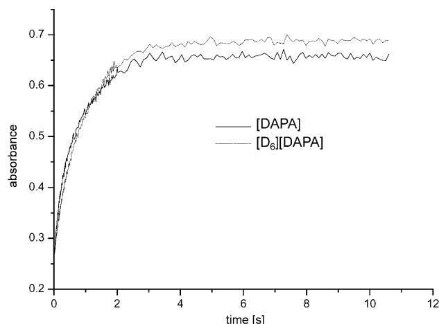
Figure 10. Absorbance during oxygenation of 1a at 353 nm in methanol. T = -60.1\text{ }^{\circ}\text{C} ; [\text{DAPA}] = 0.1\text{ mM} ; [\text{D}_6][\text{DAPA}] = 0.1\text{ mM} ; [\text{O}_2] = 4.25\text{ mM} ; t = 10.6\text{ s} .
