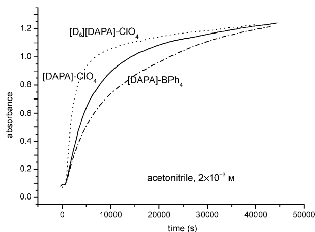
Figure 11. Absorbance at 358 nm for 1b (solid), 1D (dotted), and 1c (dash-dotted) during oxygenation in acetonitrile.
