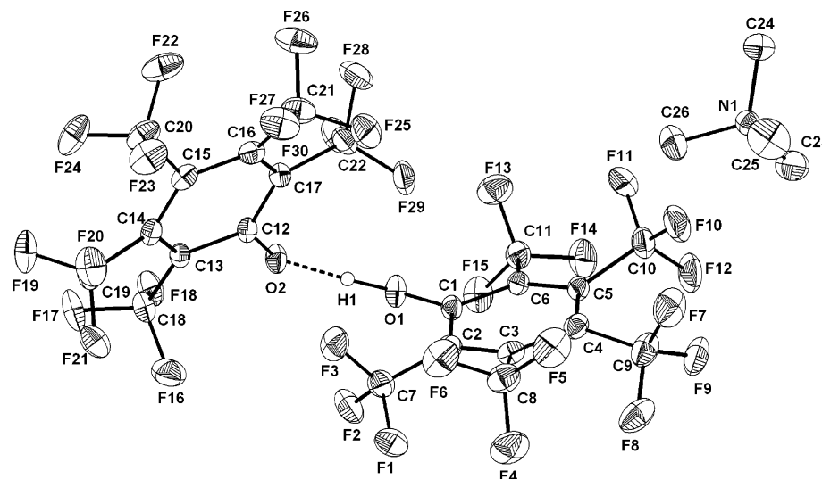
FIGURE 1. Molecular structure of 1a1 · Me 4 N + with 20% thermal ellipsoids (hydrogen atoms of Me 4 N + cation are omitted for clarity). Selected bond distances (Å) and angles (deg): O1–C1 1.305(4), O2–C12 1.289(3), C1–O1–H1 123.24(30), O1–C1–C2 124.04(27), O1–C1–C6 117.24(24), O2–C12–C17 122.97(27), O2–C12–C13 118.88(24).
