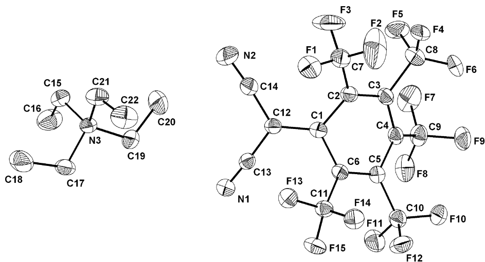
FIGURE 2. Molecular structure of 7a · \text{Et}_4\text{N}^+ with 50% thermal ellipsoids (hydrogen atoms of \text{Et}_4\text{N}^+ cation are omitted for clarity, other view of the same molecule to demonstrate distortions is in Supporting Information, Figure S4). Selected bond distances (Å), angles (deg) and dihedral angles (deg): C1–C12 1.390(2), C1–C2 1.447(2), C1–C6 1.452(2), C2–C1–C6 112.15(12), C3–C4–C5 116.87(13), C13–C12–C14 112.25(12), C14–C12–C1–C2 -4.27(24) , C1–C2–C3–C4 -11.92(21) , C1–C6–C5–C4 9.09(20).
