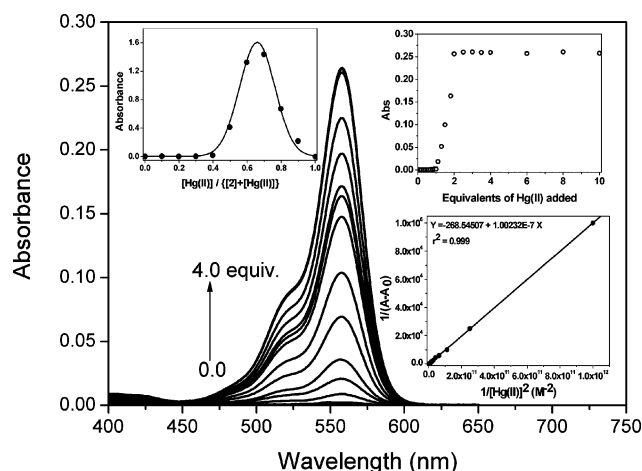
Fig. 5 Absorption spectra of the titration of 2 ( 1 \times 10^{-5} M) with different amount of Hg(II) added in MeCN–H 2 O (1 : 1 v/v). Inset: Jobs plot, absorption as a function of Hg(II) added and change in absorption of 2 at 557 nm as a function of Hg(II) concentration.
