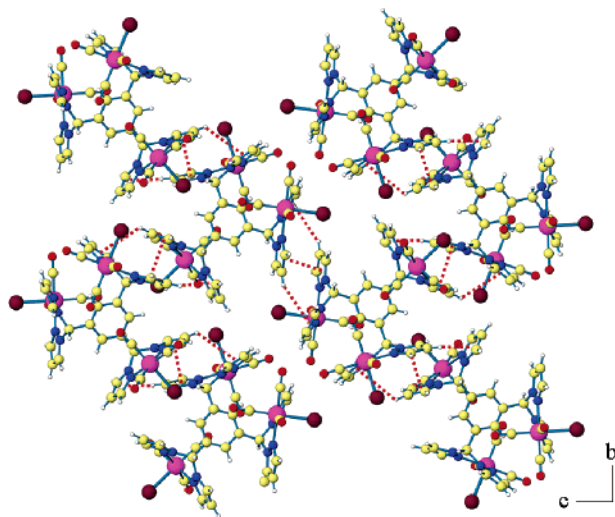
Figure 14. View of the bc -plane in 3 \cdot 3(\text{CH}_3)_2\text{CO} organized by quadruple pyrazolyl embrace interactions (red dashed lines).
