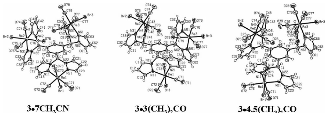
Figure 9. ORTEP drawings of the trimetallic molecules of \{\mu\text{-}1,3,5\text{-C}_6\text{H}_3[\text{CH}(\text{pz})_2]_3\}[\text{Re}(\text{CO})_3\text{Br}]_3 \cdot 7\text{CH}_3\text{CN} ( 3·7CH 3 CN ), \{\mu\text{-}1,3,5\text{-C}_6\text{H}_3[\text{CH}(\text{pz})_2]_3\}[\text{Re}(\text{CO})_3\text{Br}]_3 \cdot 3(\text{CH}_3)_2\text{CO} ( 3·3(CH 3 ) 2 CO ), and \{\mu\text{-}1,3,5\text{-C}_6\text{H}_3[\text{CH}(\text{pz})_2]_3\}[\text{Re}(\text{CO})_3\text{Br}]_3 \cdot 4.5(\text{CH}_3)_2\text{CO} ( 3·4.5(CH 3 ) 2 CO ). Ellipsoids are drawn at the 50% probability level.
