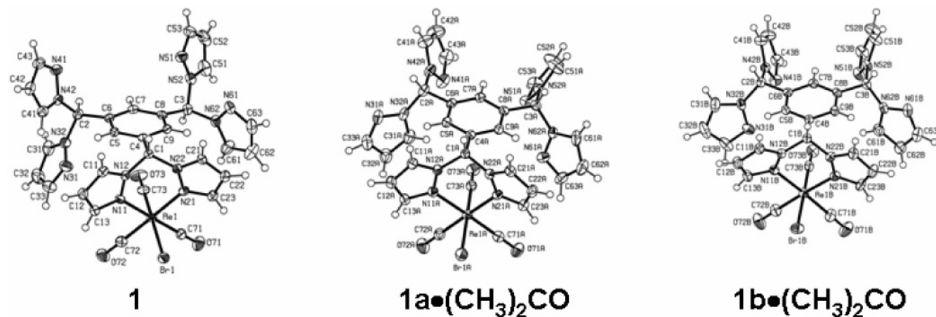
Figure 2. ORTEP drawings of the monometallic molecules of {1,3,5-[CH(pz) 2 ] 3 C 6 H 3 }Re(CO) 3 Br ( 1 ) and {1,3,5-[CH(pz) 2 ] 3 C 6 H 3 }Re(CO) 3 -Br·(CH 3 ) 2 CO ( 1 ·(CH 3 ) 2 CO). The two crystallographically independent molecules of 1 ·(CH 3 ) 2 CO are labeled 1a ·(CH 3 ) 2 CO and 1b ·(CH 3 ) 2 CO. Ellipsoids are drawn at the 50% probability level.
