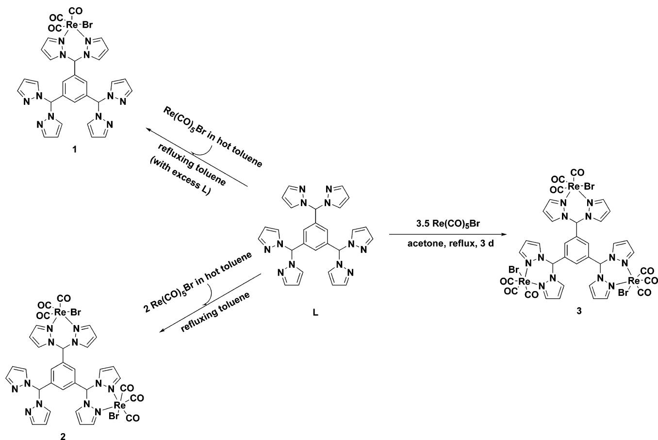
Scheme 2
