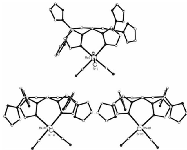
Figure 3. Comparison of the relative conformations of 1 (top) and 1 ·(CH 3 ) 2 CO (bottom) as viewed in the plane of the connecting arene rings. The two crystallographically independent molecules of 1 ·(CH 3 ) 2 CO are shown. Hydrogen atoms are omitted.
