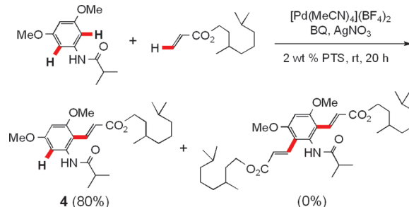
Scheme 4. Selective Coupling
