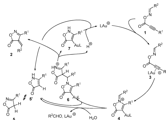
Scheme 2. Proposed Mechanism
