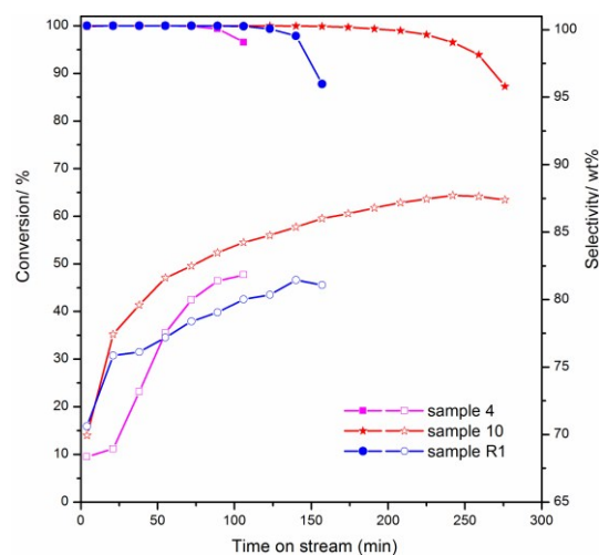
Figure 6 Methanol conversion (solid) and (\text{C}_2\text{H}_4+\text{C}_3\text{H}_6) selectivity (hollow) during the MTO reaction on samples 4, 10 and R1 (reaction conditions: 723 K, \text{CH}_3\text{OH} WHSV=4 \text{h}^{-1} , 40 wt% methanol solution).
