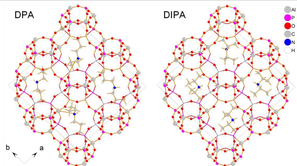
Figure 4. Optimal distributions of DPA and DIPA molecules inside the CHA cages of SAPO-34 (viewed along [001] direction).
