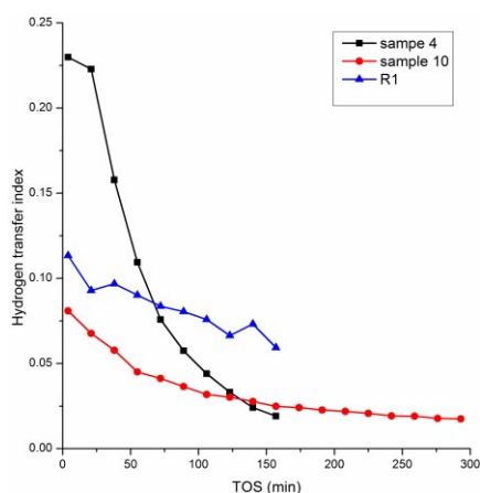
Figure 8 Hydrogen transfer index (HTI, defined as C 3 H 8 /C 3 H 6 ) of methanol conversion over the investigated catalysts.
