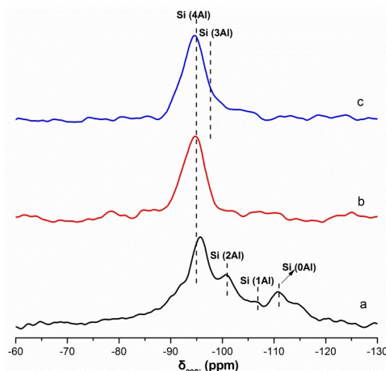
Figure 5 29 Si MAS NMR spectra of the calcined samples 4 (a), 10 (b) and R1 (c)
