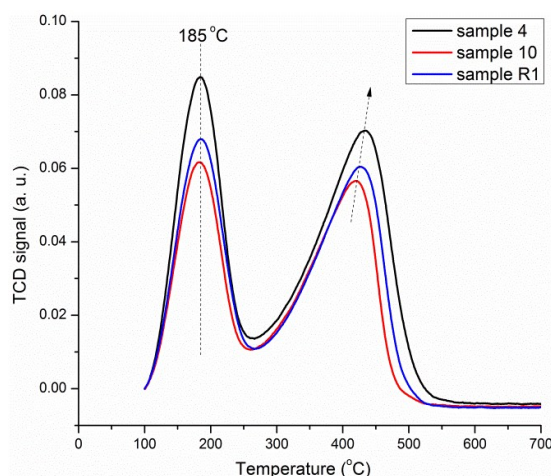
Figure 7 Temperature programmed desorption curves of ammonia for the calcined samples 4, 10 and R1.
