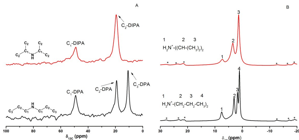
Figure 2. ^{13}\text{C} MAS NMR (A) and ^1\text{H} MAS NMR (B) spectra of the as-synthesized samples 4 (below) and 10 (above); Asterisks indicate spinning sidebands.
