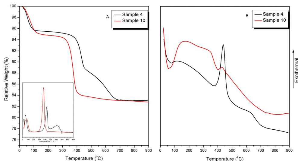
Figure 3. TG (A) and DSC (B) curves of the as-synthesized samples of 4 and 10; the corresponding DTG curves of the two samples are also presented (inset, A)
