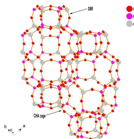
Figure 1 The barrel-like cages of SAPO-34 (Si omitted); two CHA cages are shown in the structure
