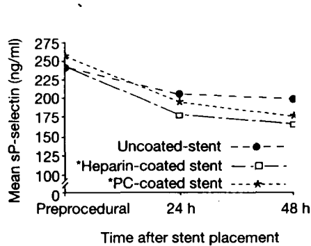
FIG. 1 Time course of plasma sP-selectin levels in patients undergoing implantation of intracoronary uncoated, PC-coated, and heparin-coated stents. (*p<0.05. vs. baseline). PC = phosphorylcholine.
