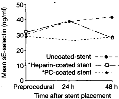
FIG. 2 Time course of plasma sE-selectin levels in patients undergoing implantation of intracoronary uncoated, PC-coated, and heparin-coated stents. (*p<0.05. vs. baseline). Abbreviation as in Figure 1.
