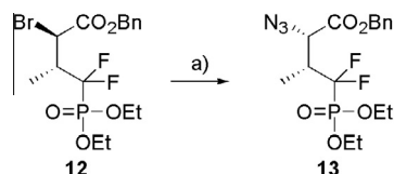
Scheme 4. Preparation of synthetic intermediate 13 . Reagents and conditions: (a) tetrabutylammonium azide, MeCN, 0 °C, 51%.
