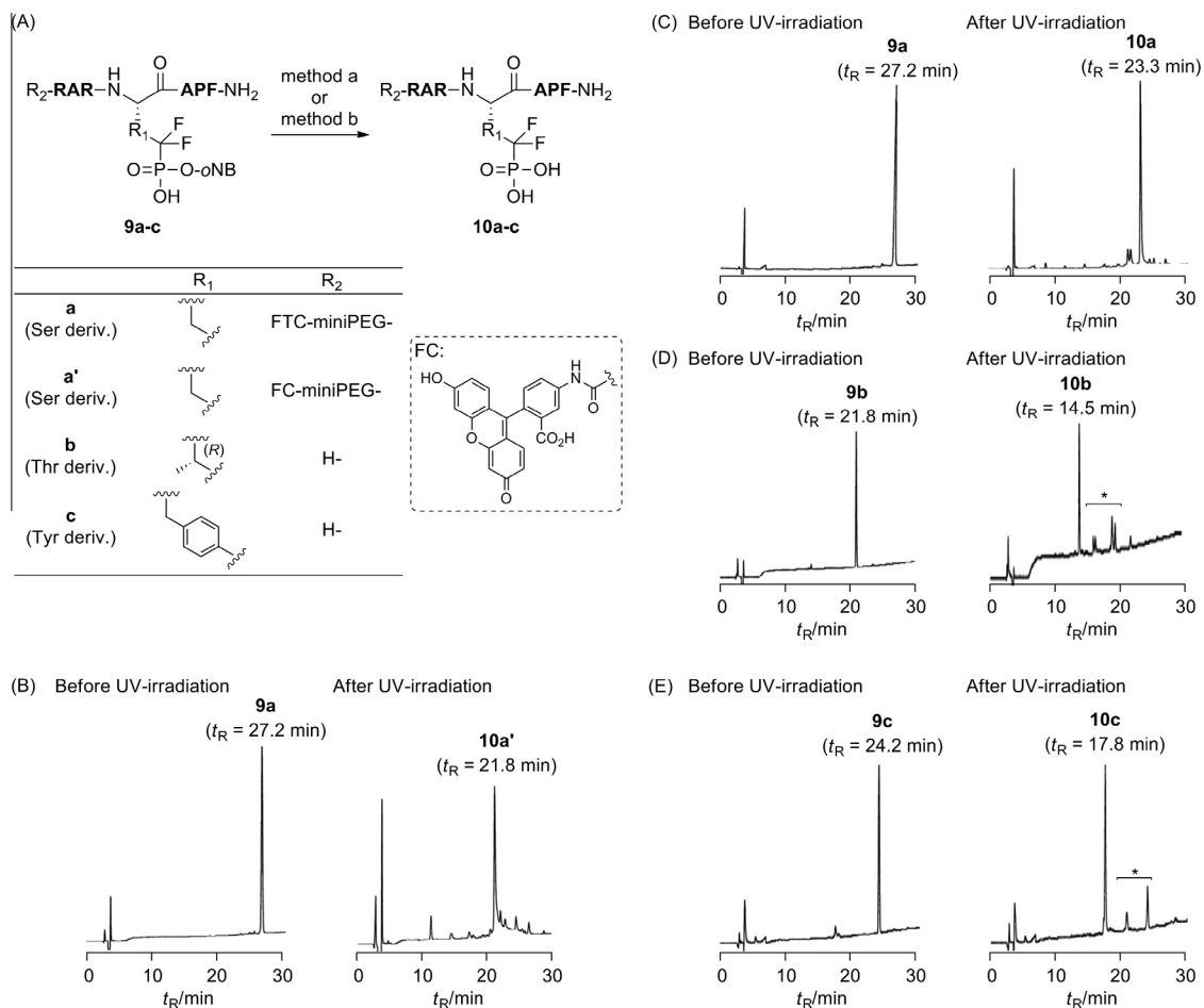
Figure 1. Photo-irradiation reactions. (A) Reagents and conditions: method (a) UV-irradiation (>365 nm, 7 min) in sodium phosphate buffer (10 mM, pH 7.6); method (b) UV irradiation (>365 nm, 7 min) in 0.1% (v/v) aqueous solution of TFA. (B–E) Analytical HPLC profiles of reaction of peptide 9a (B: method a; C: method b), 9b (D: method a), and 9c (E: method a), before and after UV irradiation. *Non-peptidyl peaks. HPLC conditions: linear gradient of 0.1% (v/v) TFA/MeCN in 0.1% (v/v) TFA aq, 10–45% (B and C) or 5–45% (D and E) over 30 min.
