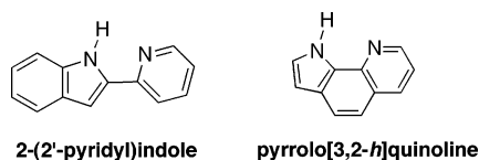
Figure 1. Precursors to unsymmetrical monoanionic nitrogen-based ligands.
