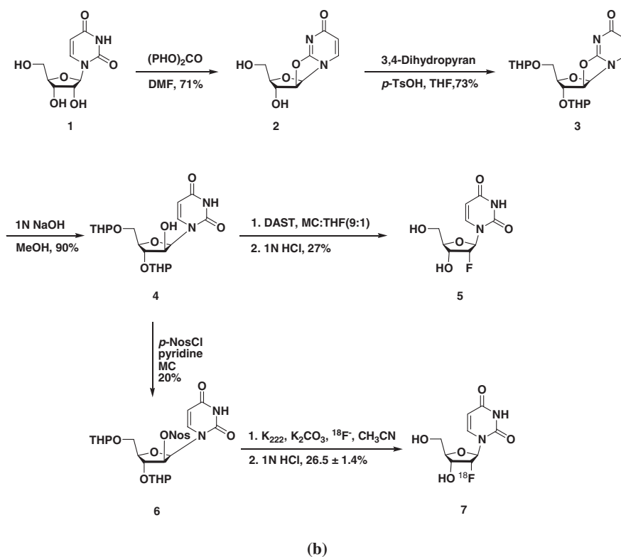
Scheme 1. Chemical and radiochemical synthesis of the precursor and 2'-[ 18 F]FU. The precursor, 3',5'-di- O -tetrahydropyranyl-2'- O -nosyl-1-β- D -arabinopentofuranosyluracil, was synthesized from uridine in four steps, and [ 18 F]2'-FU was obtained from the precursor in two steps ([ 18 F]fluorination and hydrolysis of protecting groups)
