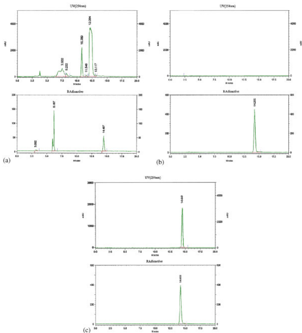
Figure 2. Purification of 2'-[ ^{18}\text{F} ]FU: (a) HPLC profile of 2'-[ ^{18}\text{F} ]FU (14.4 min) after crude HPLC purification; and (b) HPLC chromatogram of HPLC-purified 2'-[ ^{18}\text{F} ]FU; and (c) HPLC chromatogram of coinjected purified 2'-FU and 2'-[ ^{18}\text{F} ]FU. Unlike the TLC results, there were three radioactive peaks in the HPLC profile of the crude sample (a). Upper chromatogram shows UV detection, and lower chromatogram shows radioactivity. In (c) the retention times of 2'-FU and 2'-[ ^{18}\text{F} ]FU were the same
