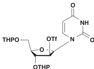
Figure 1. Chemical structure of the triflate precursor, 3',5'-di- O -tetrahydropyranyl-2'- O -triflate-1- \beta -D-arabinopentofuranosyluracil. In the previous report, this triflate leaving group procedure showed high [ ^{18}\text{F} ]fluorination yields but very low chemical stability even below 0^\circ\text{C} 11
