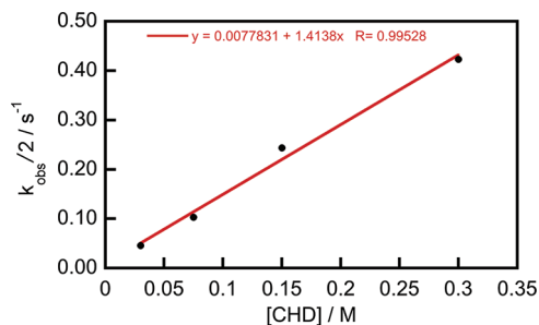
Figure 8. Plot of k_{\text{obs}}/2 vs [\text{CHD}] for the reaction of 5 with CHD at -30^\circ \text{C} . The second-order rate constant is obtained from the slope to be 1.4 \text{ M}^{-1} \text{ s}^{-1} .
