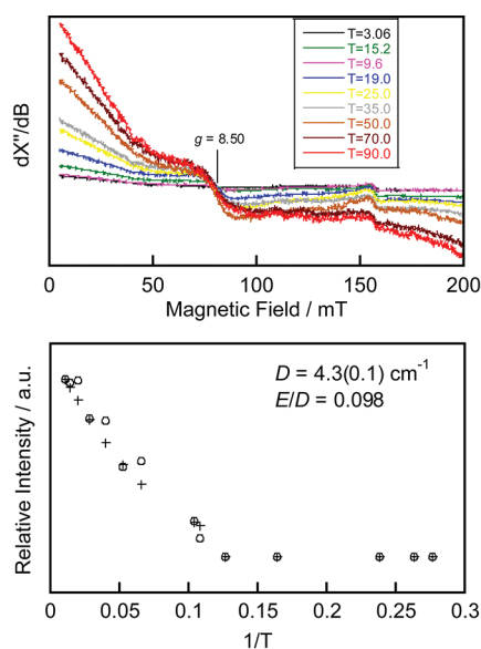
Figure 6. Temperature dependence of parallel-mode EPR spectrum of 5 from 3 to 90 K (top). Relative intensity of g = 8.50 feature versus 1/T for experimental (○) and calculated (+) spectra (bottom). Best fit analysis provides a value for the axial zero-field splitting parameter, D , of 4.3 \text{ cm}^{-1} .
