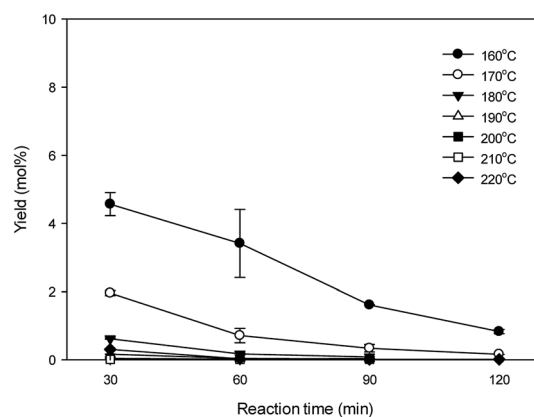
(A) 5-HMF
