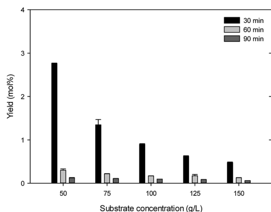
(A) 5-HMF
