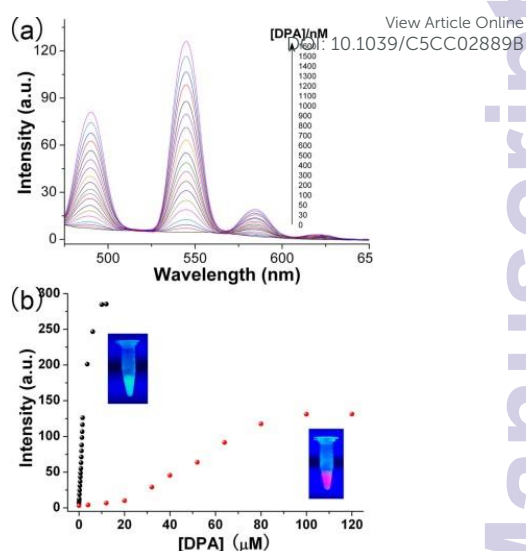
Figure 2. (a) Fluorescence response of 4 μgml -1 GE-Tb upon addition of different concentrations of DPA. (b) The fluorescence intensity of GE-Tb (545 nm, black) or GE-Eu (610 nm, red) as a function of DPA concentration. Inset: Photographs of GE-Tb-DPA (green) or GE-Eu-DPA (red) taken under 365 nm UV light.
