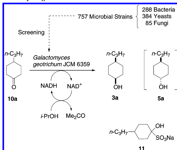
Scheme 2. Reduction of 4-propylcyclohexanone 10a with Galactomyces geotrichum JCM 6359
