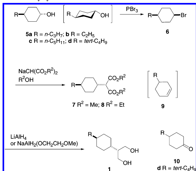
Scheme 1. Existing route to trans -2-(4-alkylcyclohexyl)-1,3-propanediol 1 from trans -4-alkylcyclohexanol 5
