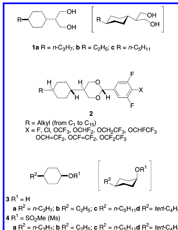
Figure 1. Structures of trans -2-(4-alkylcyclohexyl)-1,3-propanediol 1 , its derived liquid-crystal 2 , cis -4-alkylcyclohexanol 3 , and cis -4-alkylcyclohexyl mesylate 4 .
