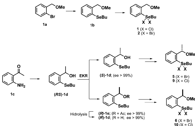
Scheme 1 Synthesis of organoselenananes 1–2, 5–6 and 9–10. 12a
