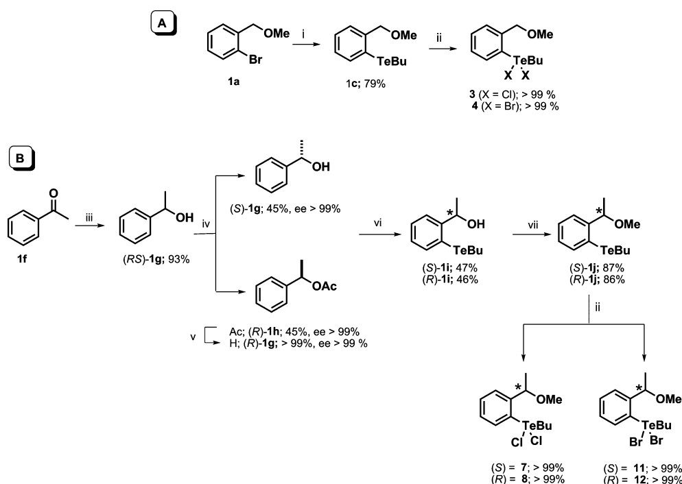
Scheme 2 Reagents and conditions: (i) a: t -BuLi, THF (−78–0 °C, 30 min); b: BuTeTeBu (r.t., 3 h); (ii) SO 2 Cl 2 or Br 2 , THF (0 °C, 15 min); (iii) NaBH 4 , MeOH (r.t., 1 h); (iv) vinyl acetate, CAL-B, hexane (32 °C, 7 h); (v) K 2 CO 3 , MeOH, H 2 O (r.t. overnight); (vi) a: n -BuLi, TMEDA, pentane (reflux, 24 h), b: BuTeTeBu (0 °C – r.t., 2 h); (vii) a: NaH, THF (0 °C, 30 min), b: MeI (r.t., 2 h).
