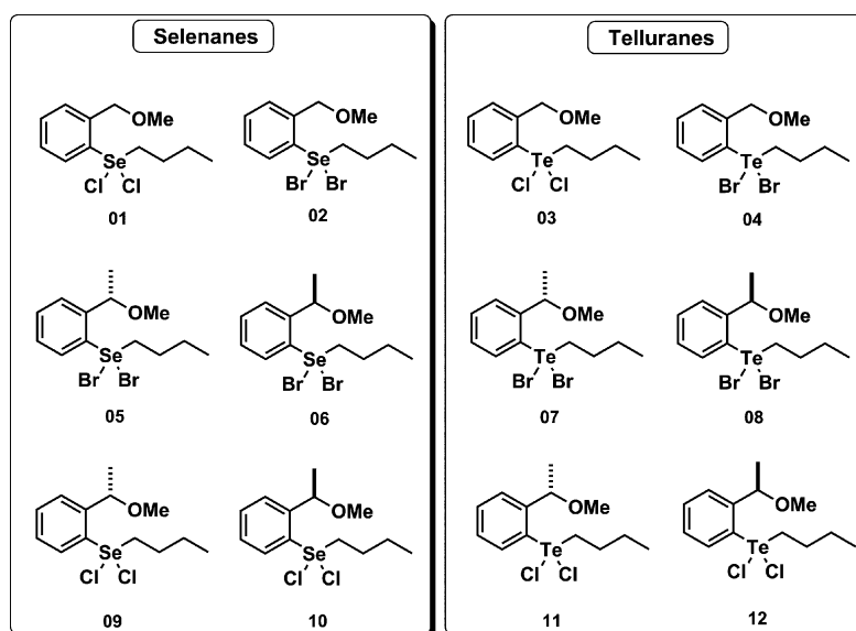
Fig. 1 Selenananes and tellurananes evaluated as inhibitors of Protein Tyrosin Phosphatase.
