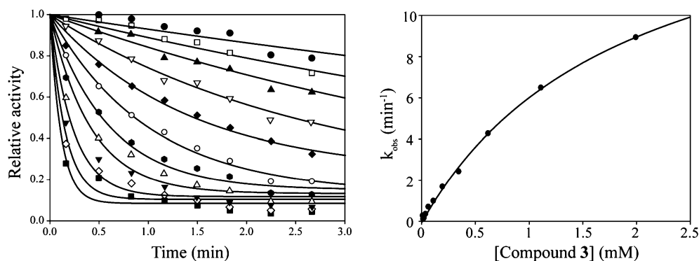
Fig. 2 Kinetic analysis of PTP1B inactivation by 3 at 25 °C and pH 7. Panel on the left: time and concentration dependence of inhibitor 3 -mediated PTP1B inactivation. Compound 3 concentrations were as follows: ● 6 μM, □ 10 μM, ▲ 18 μM, ▽ 33 μM, ◆ 59 μM, ○ 106 μM, ● 190 μM, △ 343 μM, ▽ 617 μM, ◇ 1111 μM, and ■ 2000 μM. Panel on the right: Concentration dependence of the pseudo-first-order rate constants k_{\text{obs}} for 3 -mediated PTP1B inactivation.
