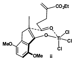
Figure 2. Plausible intermediate ii leading to highly stereocontrolled aldolization of 9 with 10 .
