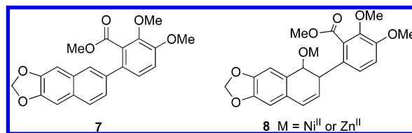
FIGURE 2. Structures of 7 and 8 .
