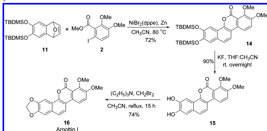
SCHEME 4. Total Synthesis of Arnottin I
