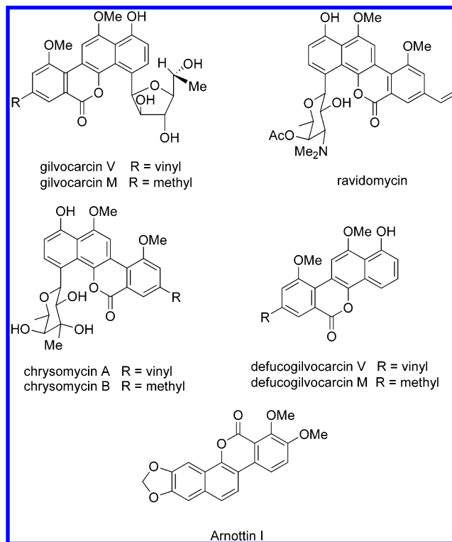
FIGURE 1. Structures of gilvocarcin-class antibiotics.
