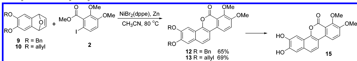
SCHEME 4. Total Synthesis of Arnottin I
