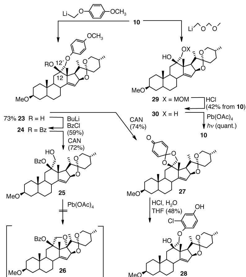
Scheme 4. Attempts towards Heptacycle 26 . CAN = \text{Ce}(\text{NH}_4)_2(\text{NO}_3)_6 , MOM = \text{MeOCH}_2
