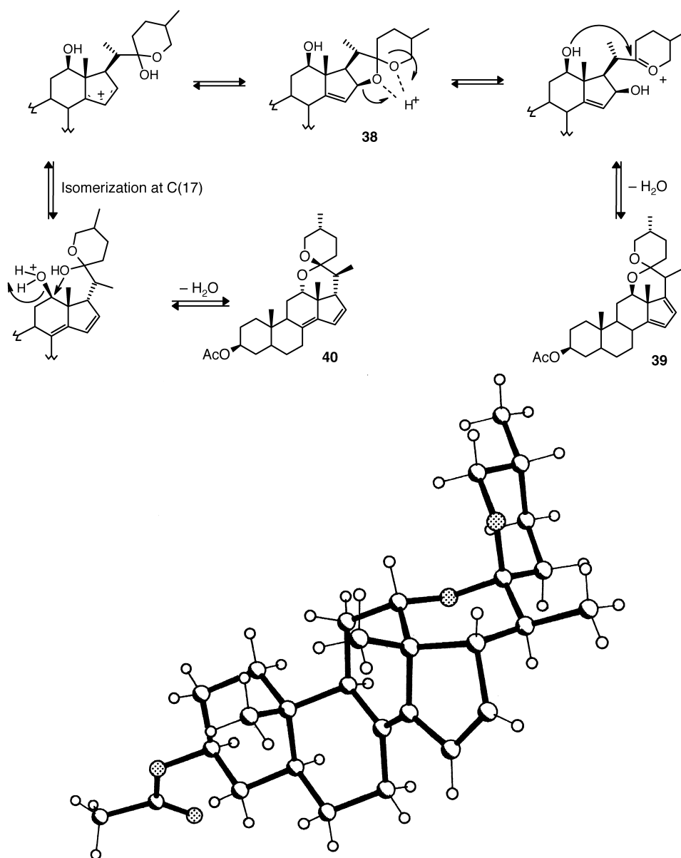
Fig. 2. X-Ray structure of dienyl acetate 40
