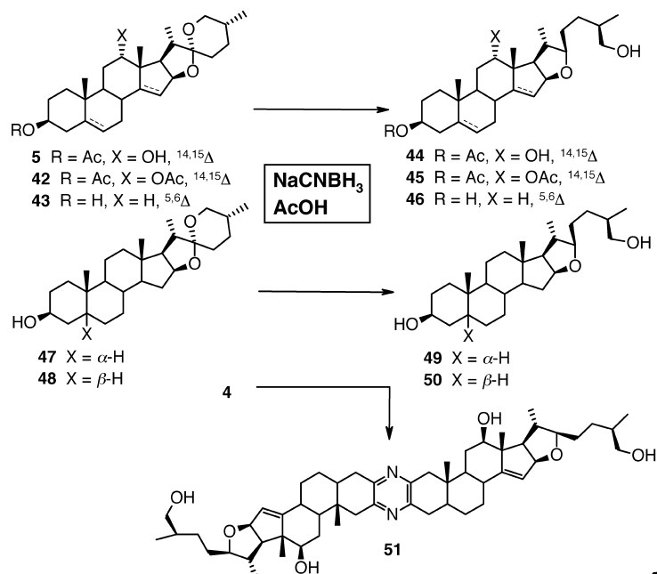
Scheme 9. Novel Reductive Opening of Sapogenin Spiroketal
