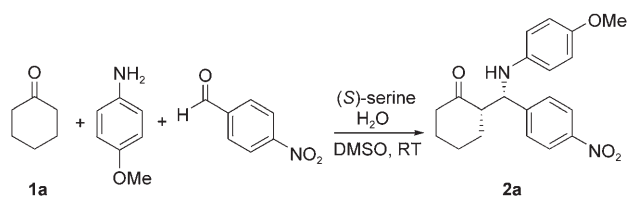
Scheme 1. The reaction of cyclohexanone 1a (1.5 mmol), p -nitrobenzaldehyde (0.50 mmol), p -anisidine (0.45 mmol), H 2 O (1 mmol, 18 \mu L, 2 equiv), [17] serine (30 mol %), and dimethylsulfoxide (DMSO; 2 mL) for 48 h produced the corresponding Mannich product 2a in a 60% yield with 6:1 d.r. ( syn/anti ) and 94% ee .
