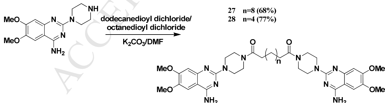
Scheme 3. Synthesis of dimer 27 and 28
