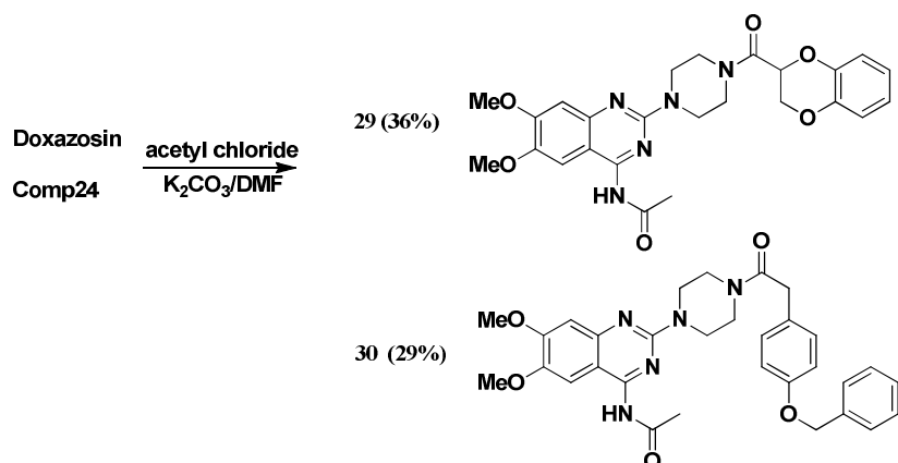
Scheme 4. Synthesis of B moiety acetylated analogs
