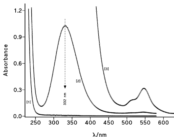
Fig. 1 UV–visible spectra of [1] cap 2.9 mM at [H^+] = 0.05 \text{ M} ; [2] NOcap formed in the reaction sample of [nit] = 1.0 \text{ mM} , [cap] = 2.9 \text{ mM} , and [H^+] = 0.050 \text{ M} ; and [3] NOcap formed in the reaction sample of [cap] = [nit] = 0.012 \text{ M} and [H^+] = 0.060 \text{ M} .
