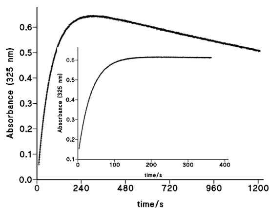
Fig. 7 Plot of absorbance readings at 325 nm against time for the reaction of cap 12.7 mM and tBN 1.1 mM in aqueous basic medium of 0.085 M carbonate-bicarbonate buffer of pH 10.1, A-t data fits perfectly to A = A_\infty + C_1 \cdot \exp(-k_1 t) + C_2 \cdot \exp(-k_2 t) , the plot contains 1000 experimental points and the solid line (undistinguishable) of the fit process passes through every point; the inset shows the same plot for the reaction of 12.7 mM cap and 1.1 mM tBN in alkaline medium of [\text{OH}^-] = 0.14 \text{ M} , but the A-t data fits perfectly to A = A_\infty - (A_0 - A_\infty) \cdot \exp(-k_1 t) .
