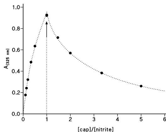
Fig. 2 Stoichiometric plot of the reaction of nit and cap in aqueous perchloric acid 0.050 M showing the variation of the absorbance readings at the end of the reaction for [cap] = [nit] = 2 \text{ mM} mixed at different concentration ratios.
