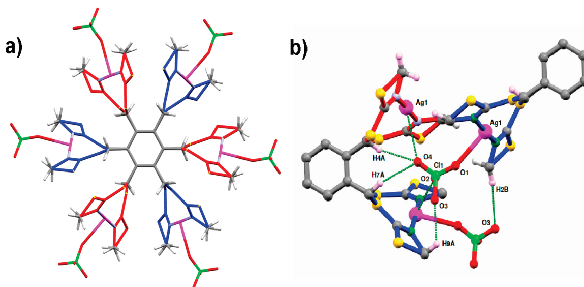
Figure 7. (a) Perspective view of cleft binding \text{ClO}_4^- in the side pocket of metallocage 2 . (b) Partial view showing the binding interactions of \text{ClO}_4^- in the cleft pocket of metallocage 2 with hydrogen bonding parameters C4...H4A...O4 (C4...O4 = 3.307 Å, \angle\text{C4-H4A}\cdots\text{O4} = 150.0^\circ ), C7...H7A...O4 (C7...O4 = 3.453 Å, \angle\text{C7-H7A}\cdots\text{O4} = 142.54^\circ ), C9...H9A...O3 (C9...O3 = 3.078 Å, \angle\text{C9-H9A}\cdots\text{O3} = 121.53^\circ ), Ag1–O2 = 3.056(7) Å, and Ag1–O4 = 3.170(9) Å.
