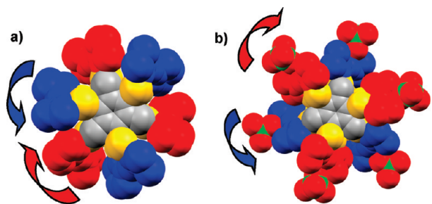
Figure 8. Perspective views of helicity in (a) metallogage 1 and (b) metallogage 2. Color code: red, atoms above the plane; blue, atoms below the plane of the central benzene ring.
