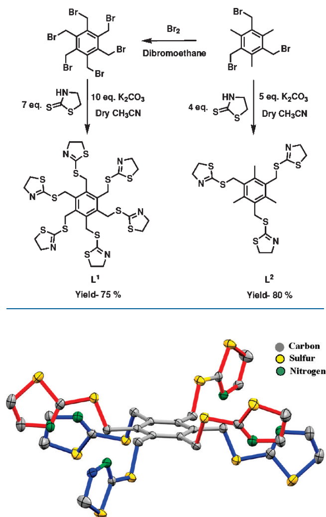
Figure 1. Perspective thermal ellipsoid view of L^1 at 50% probability. Color code: Red, atoms above the plane; blue, atoms below the plane of central benzene ring. Hydrogen atoms are omitted for clarity.
