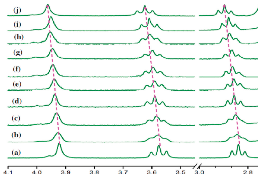
Figure 11. ^1\text{H} NMR (300 MHz) spectral changes of \text{L}^1 with added \text{AgClO}_4 in \text{CDCl}_3 – \text{DMSO}-d_6 (3:2; 25 °C; [\text{L}^1]^0 = 4.69 \text{ mM} ). Equivalents of \text{AgClO}_4 : (a) 0, (b) 0.5, (c) 1, (d) 1.5, (e) 2, (f) 2.5, (g) 3, (h) 3.5, (i) 4, (j) 4.5.
