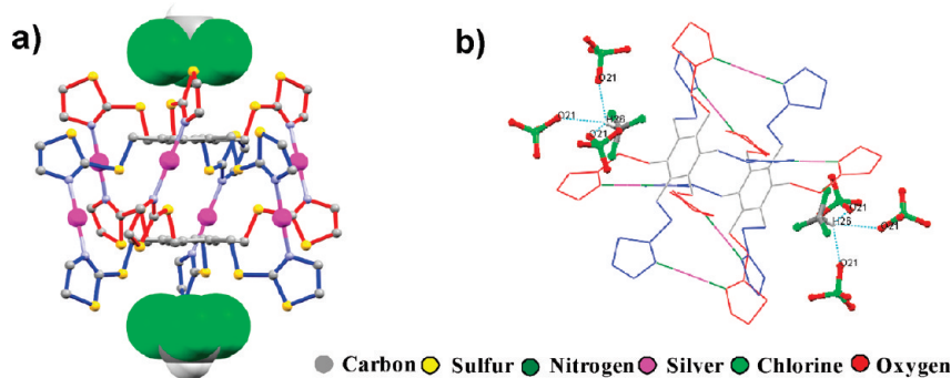
Figure 5. (a) Perspective view of metallocapsule 1 with cleft bound \text{ClO}_4^- at the side pockets and \text{CHCl}_3 at the top and bottom cavities. (b) Hydrogen bonding interactions of \text{CHCl}_3 with cleft bound perchlorate anions in 1 with a C26...O21 bond distance of 3.068 Å. Color code: red, atoms above the plane; blue, atoms below the plane of central benzene ring.
