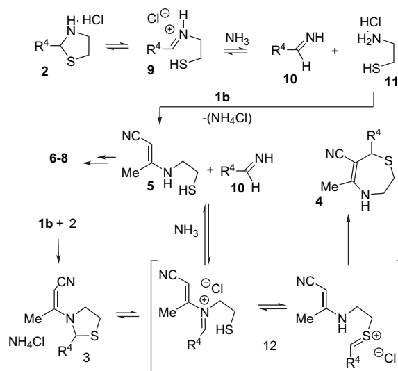
Scheme 6.
