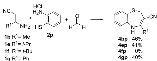
Scheme 9.
