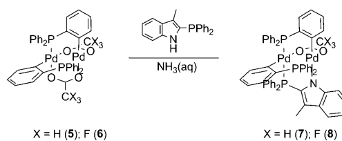
Scheme 4. Synthesis of [Pd 2 (μ-C 6 H 4 PPh 2 ) 2 (μ-C 9 H 7 NPPh 2 )(μ-O 2 CCX 3 )] (X = H ( 7 ); X = F ( 8 )).
