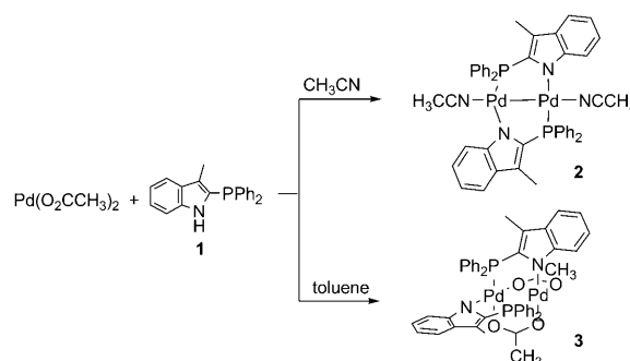
Scheme 2. Synthesis of [Pd(μ-C 9 H 7 NPPH 2 )(NCCH 3 ) 2 ] 2 and [Pd(μ-C 9 H 7 NPPH 2 )(μ-O 2 CCH 3 ) 2 ] 2 .
