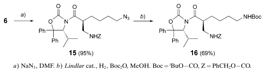
Scheme 5. ( S )- \beta^2 hLys Derivatives 15 and 16 from the Bromoalkyl Precursor 6 by Br/ N_3 -Substitution as Key Step
