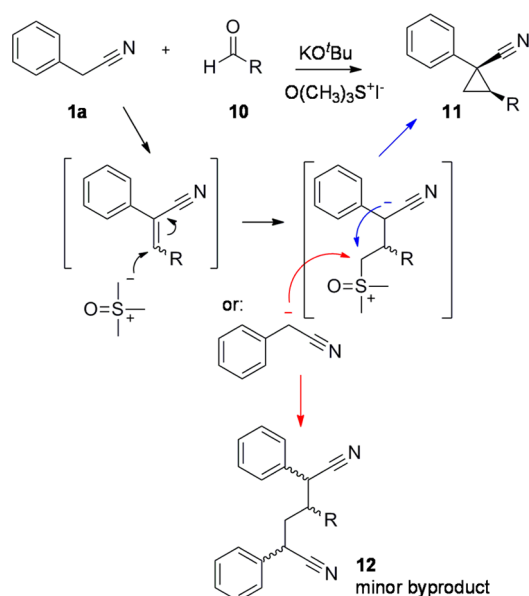
Scheme 3. Proposed Mechanism for the Formation of Product 11 and Minor Byproduct 12
