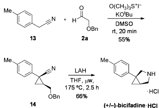
Scheme 4. Two-Step Synthesis of (±)-Bicifadine Utilizing the One-Pot Knoevenagel Condensation/Corey–Chaykovsky Cyclopropanation Reaction
