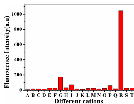
Figure 5. Fluorescence intensity of L in presence of different metal ions (at \lambda_{\text{em}} = 572 \text{ nm} ). (A) probe ( L ), (B) \text{Co}^{2+} , (C) \text{Mn}^{2+} , (D) \text{Al}^{3+} , (E) \text{Fe}^{2+} , (F) \text{Mg}^{2+} , (G) \text{Hg}^{2+} , (H) \text{K}^+ , (I) \text{Pb}^{2+} , (J) \text{Na}^+ , (K) \text{Fe}^{3+} , (L) \text{Cd}^{2+} , (M) \text{Cr}^{3+} , (N) \text{Ba}^{2+} , (O) \text{Ni}^{2+} , (P) \text{Zn}^{2+} , (Q) \text{Ca}^{2+} , (R) \text{Cu}^{2+} , (S) \text{Ag}^+ , and (T) \text{Au}^{3+} .
