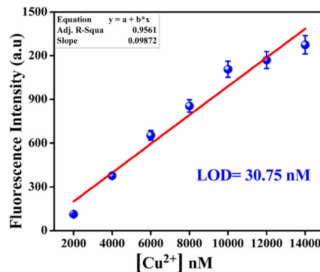
Figure 6. Calibration curve (with error bars) in the nanomolar range to calculate the LOD of \text{Cu}^{2+} ions using L from the fluorimetric titration data (at \lambda_{\text{em}} = 572 \text{ nm} ).
