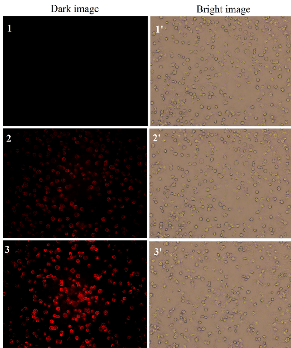
Figure 7. Fluorescence and bright field images of AGS cells after incubation with L (20 \mu M) followed by addition of \text{Cu}^{2+} ions, (1, 1') 0 \mu M, (2, 2') 10 \mu M and (3, 3') 20 \mu M, respectively. All the samples were excited at 550 nm by using a [63X] objective.
