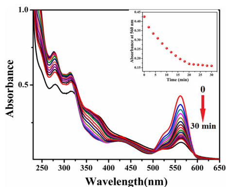
Figure 4. UV-Vis spectra of L in presence of \text{Cu}^{2+} ions (1.0 equiv.) with increase in time. (Inset) Plot of Absorbance of L (at \lambda_{\text{max}} = 560 \text{ nm} ) in presence of \text{Cu}^{2+} ions vs. Time.
