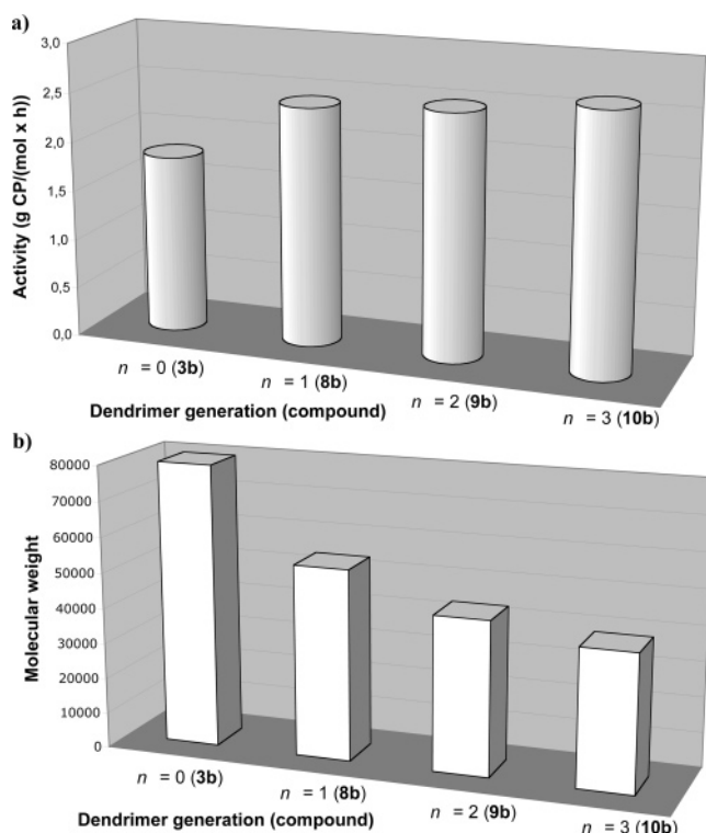
Figure 3. (a) Activities for Gn -ONNMe 2 [Pd(MeCN)Me] + and (b) copolymer M w values obtained using neat TBS as a solvent.
