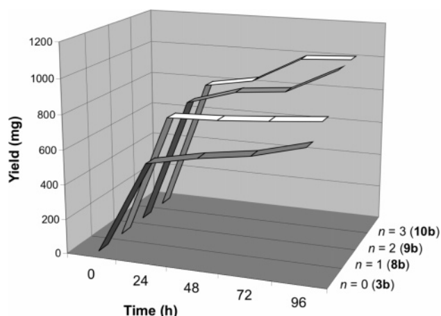
Figure 4. Effect of time on yield of copolymer produced by compounds Gn -ONNMe 2 [Pd(L)Me] + in neat TBS.
