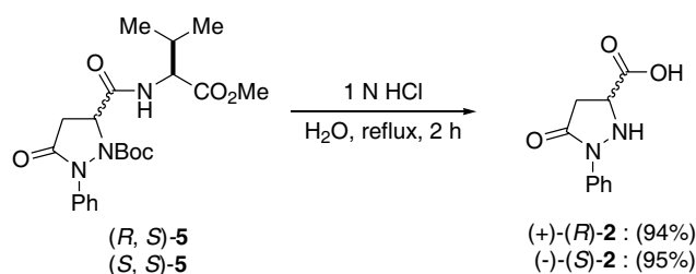
Scheme II The acidic hydrolysis and deprotection of diastereomer ( R,S )-5 and ( S,S )-5
