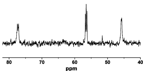
Figure 6. ^{31}P\{^1H\} NMR spectrum (161 MHz, CD_2Cl_2 , 20 °C) of 3 . Signals at \delta 77 and 45 are assigned to dppe, the signal at \delta 55 is assigned to PPh_3 .
