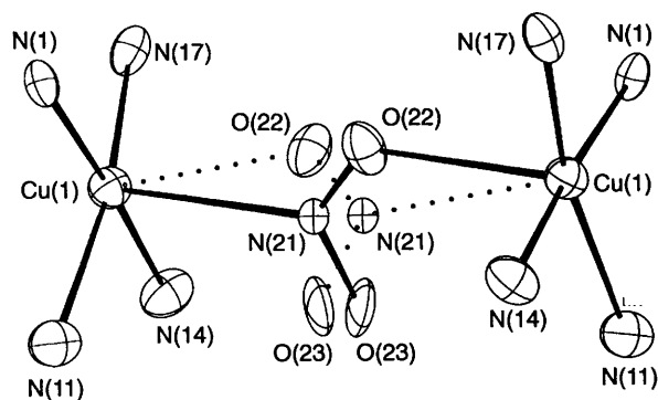
Fig. 3 Detail of the structure of 7 showing the geometry and disorder of the \mu -nitrito- \kappa\text{O}:\kappa\text{N} bridge
