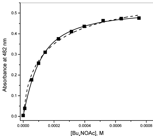
FIGURE 4. Titration curve for 7.0 \times 10^{-5} M 3 (absorbance at 482 nm) with Bu 4 NOAc in DMSO. Solid line: formal fit to eq 8. Dashed line: fit to eqs 1–3 (see text for details).
