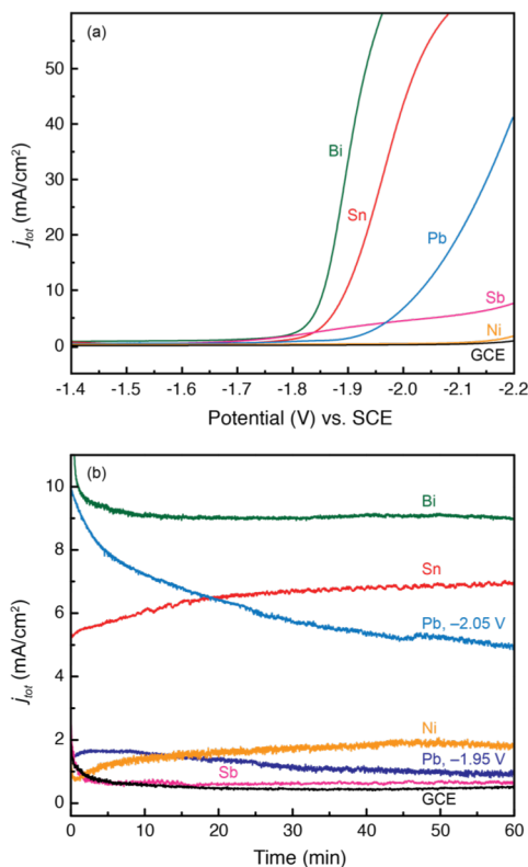
Figure 3. (a) Linear sweep voltammograms (LSVs) and (b) total current density profiles recorded for electrodeposited cathode materials in CO 2 saturated MeCN containing 100 mM [BMIM]OTf. Current density plots for which no potential is listed were recorded at −1.95 V versus SCE.
