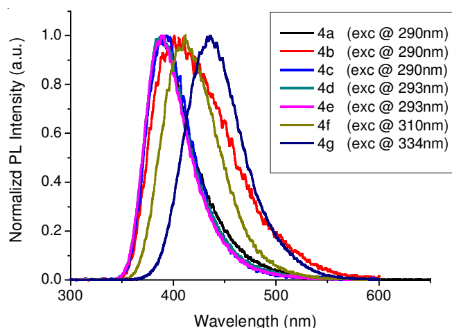
Fig. 2. Emission spectra of the 4a-4g in acetonitrile solution ( \lambda_{\text{ex}} = \lambda_{\text{UV-max}} )
