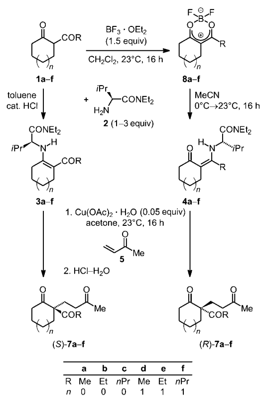
Scheme 2. Preparation of endo- and exocyclic enamines 3 and 4 and their use as a configuration switch in asymmetric copper(II)-catalyzed Michael reactions.
