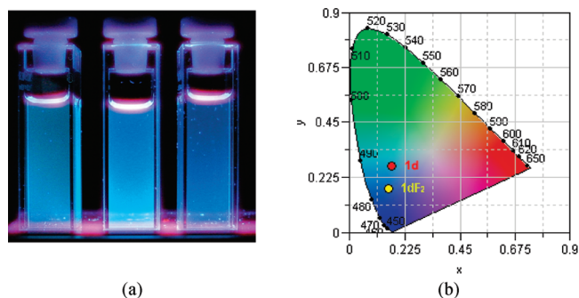
Figure 5. (a) From left, photoemission cells containing Ir(ppy)(PPh 3 ) 2 -(H)(CN) ( 1d ), Ir(F 2 ppy)(PPh 3 ) 2 (H)(CN) ( 1dF 2 ), and Ir(F 2 Meppy)(PPh 3 ) 2 -(H)(CN) ( 1dF 2 Me ) in CH 2 Cl 2 . (b) CIE coordinates for 1d and 1dF 2 ( 1dF 2 Me is not shown as it is practically the same with 1dF 2 ).
