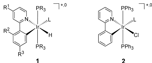
Figure 1. Chemical Structures of [\text{Ir}(\text{C}^{\text{N}})(\text{L})(\text{H})(\text{PR}_3)_2]^{0,+} ( 1 ) and [\text{Ir}(\text{ppy})(\text{L})(\text{Cl})(\text{PPh}_3)_2]^{0,+} ( 2 ).
