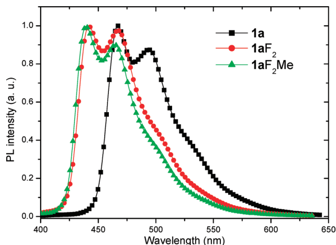
Figure 4. Normalized emission spectra of Ir(ppy)(PPh 3 ) 2 (H)(Cl) ( 1a ) (—■—), Ir(F 2 ppy)(PPh 3 ) 2 (H)(Cl) ( 1aF 2 ) (—●—), and Ir(F 2 Meppy)(PPh 3 ) 2 (H)(Cl) ( 1aF 2 Me ) (—▲—) in degassed CH 2 Cl 2 at 25 °C.
