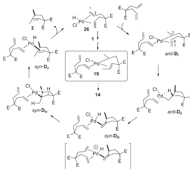
Scheme 10. A mechanism, based on kinetics, isotopic labelling, Hammett correlation, reaction of isomeric 1,5-dienes ( 14 and 23 ), and intermolecular regioselectivity control by aryl-1,6-dienes ( 9 ), for the highly regioselective cycloisomerisation of 1 → 3 by pre-catalysts of type 8 as compared to the much less selective cycloisomerisation 1 → 2 by cationic pre-catalysts of type 5 (see intermediate in square parentheses). Reaction of the pre-catalyst 8 with 1 (or with Et 3 SiH in the presence of 1 ) is proposed to initiate catalysis by generation of 26 . Turnover numbers are limited to ca. 80 per mol 26 due to a side reaction involving isomerisation 1 → 14 (not liberated)→ 19 which is rather inert towards β-H elimination (see inset to Scheme) and sequesters Pd “off-cycle”.
