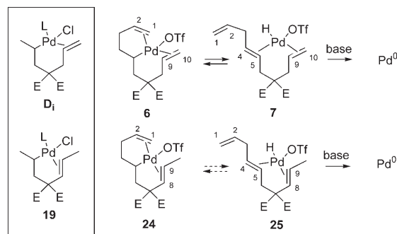
Scheme 9. Contrasting reactivities of complexes 6 and 24 towards C(1)=C(2) alkene displacement and then \beta -H elimination to generate 7 and 25 , respectively, as probed by deprotonation of the latter complexes by simple organic bases, such as a 1,8-bis(dimethylamino)naphthalene. Inset: the structural relationships of Pd complexes D i and 19 (L = alkene) to 6 and 24 , see text for full discussion.
