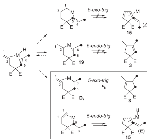
Scheme 8. Four potential pathways for cycloisomerisation on hydropalladation of the C(1)=C(2) or C(5)=C(6) double bonds of 1,5-diene ( E )- 14 , to give cycloisomers 15 or 3 depending on the regiochemistry of the hydropalladation event. The mechanisms that are consistent with the observed 13 C label distributions and double bond geometry in 3 and 15b respectively [Scheme 7 and Eqs. (j) and (k)], are shown in the boxed area. Intermediate 19 is proposed to be the mode of catalyst inhibition, see text for full discussion.
