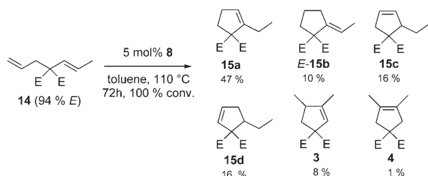
Scheme 7. Cycloisomerisation of ( E )- 14 , the regioisomer of 1,6-diene 1 , catalysed by Pd pre-catalyst 8 . Reaction of 1 proceeds significantly faster than that of ( E )- 14 when reacted alone (100 % conversion, 90 minutes, 40 °C) but when mixed in equimolar quantities with ( E )- 14 both the 1,5- and 1,6-isomers ( 14 and 1 , respectively) convert, within experimental error, at the same rate.
