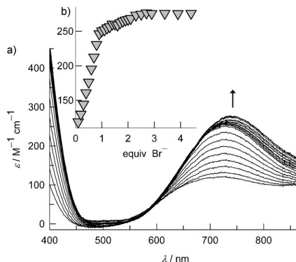
Figure 2. a) Spectra recorded in the visible region over the course of the titration of a solution of [\text{Cu}^{\text{II}}(1)]^{4+} in MeCN ( 1.01 \times 10^{-4} \text{ M} ) with a standard solution of [\text{Bu}_4\text{N}]\text{Br} in MeCN. Optical path: 1 cm; \epsilon : molar absorptance. b) Titration profile at 745 nm.
