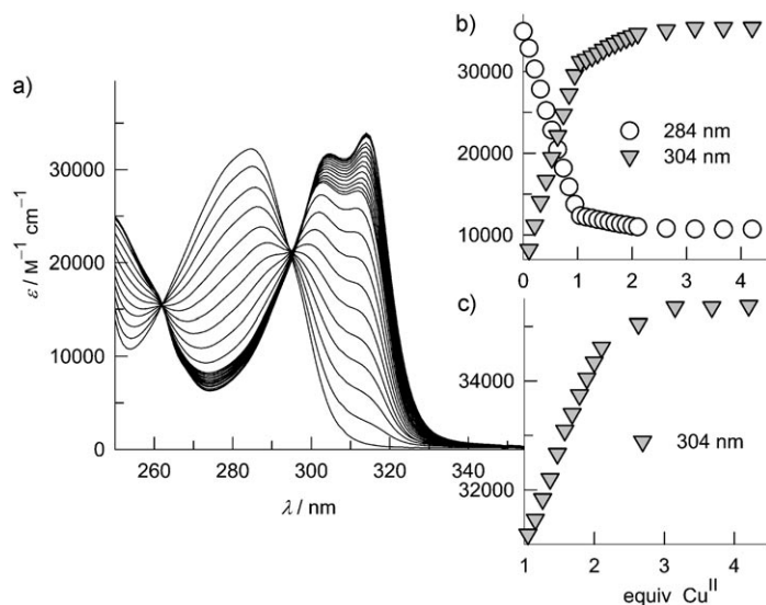
Figure 1. a) UV spectra recorded over the course of the titration of a solution of [1]^{2+} in MeCN ( 3.7 \times 10^{-4} \text{ M} ) with a standard solution of \text{Cu}^{\text{II}} ( \text{CF}_3\text{SO}_3 ) 2 in MeCN; b) titration profiles at 284 nm (○) and 304 nm (▼); and c) titration profile at 304 nm, after addition of one equivalent of \text{Cu}^{\text{II}} .
