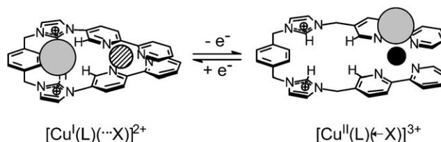
Scheme 1. The planned translocation of an anion X^- (grey sphere) within the [Cu^{II}(L)]^{4+/3+} system, driven by the Cu^{II}/Cu^I redox couple ( Cu^I : hashed sphere; Cu^{II} : black sphere). The redox change induces a change of the coordination geometry at the metal centre, from tetrahedral ( Cu^I ) to a five-coordinate arrangement ( Cu^{II} , square pyramidal or trigonal bipyramidal).
