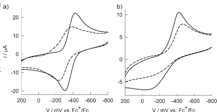
Figure 9. CV profiles obtained at the platinum working electrode (potential scan rate 500 \text{ mV s}^{-1} ) in a solution of [\text{Bu}_4\text{N}]\text{ClO}_4 in MeCN ( 0.1 \text{ M} ). a) (----) [\text{Cu}^{\text{II}}(\text{Mebpy})_2]^{2+} ( 2.00 \times 10^{-3} \text{ M} ), (—) + excess [\text{Bu}_4\text{N}]\text{NO}_3 ; b) (----) [\mathbf{1}]^{2+} and \text{Cu}^{\text{II}}(\text{CF}_3\text{SO}_3)_2 (both 1.5 \times 10^{-3} \text{ M} ); (—) + [\text{Bu}_4\text{N}]\text{NO}_3 (1.0 equiv).
