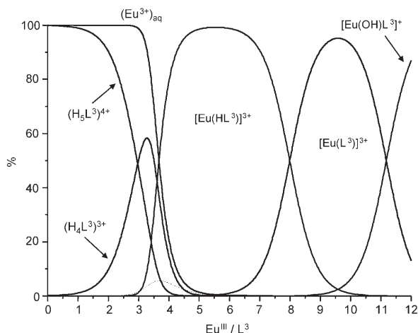
Figure 1. Distribution diagram for the system \text{Eu}^{\text{III}}/\text{L}^3 as calculated from spectrophotometric titrations in the pH range 1.92–12.24 at 25 °C and with I = 0.1 \text{ M} ( \text{Me}_4\text{NCl} ).
