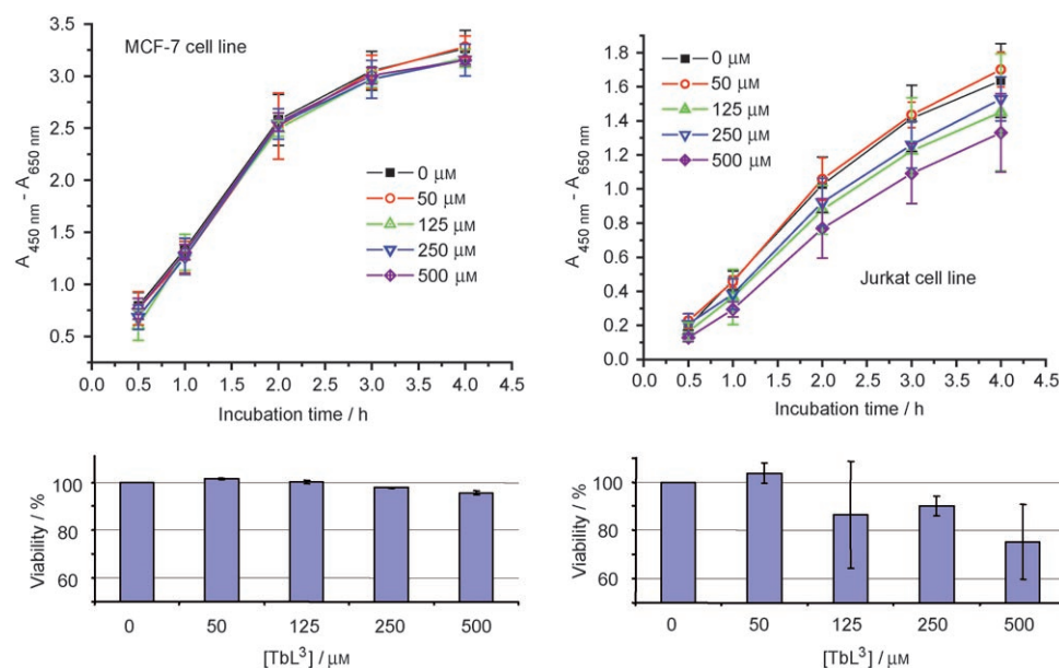
Figure 6. Top: WST-1 proliferation test of cells in the absence or presence of different concentrations of \text{TbL}^3 . Bottom: Cell viability values (%), obtained by using the same test, for different concentrations of \text{TbL}^3 after 24 h incubation at 37°C.
