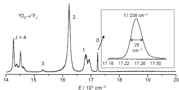
Figure 3. High-resolution emission spectrum of microcrystalline \text{EuL}^3 measured at 295 K upon ^5\text{D}_2 \rightarrow ^7\text{F}_0 excitation ( 21460 \text{ cm}^{-1} , 466 nm) and recorded in time-resolved mode. The inset shows an enlargement of the ^5\text{D}_0 \rightarrow ^7\text{F}_0 transition.
