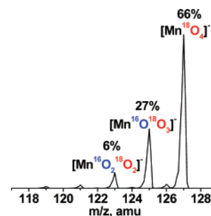
Figure 6. ESI/MS (–ve mode) of ^{18}\text{O} -labeled potassium permanganate in acetonitrile.
