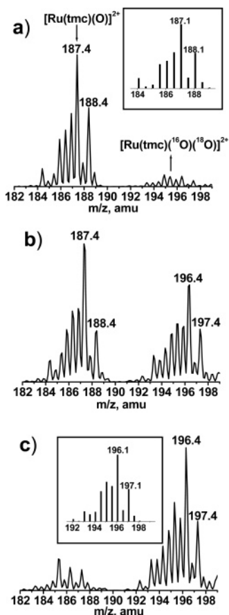
Figure 9. The ESI/MS (+ve mode) of [\text{Ru}^{\text{IV}}(\text{tmc})(\text{O})(\text{NCCH}_3)](\text{PF}_6)_2 (3 mM) and \text{K}[\text{Mn}^{18}\text{O}_4] (25 mM) in \text{CH}_3\text{CN} at different time intervals: (a) 1 h, (b) 7 h, (c) 24 h. The insets in panels a and c show the calculated isotopic patterns for [\text{Ru}(\text{tmc})(\text{O})]^{2+} and 80% [\text{Ru}(\text{tmc})(^{16}\text{O})(^{18}\text{O})]^{2+} + 20% [\text{Ru}(\text{tmc})(^{16}\text{O})_2]^{2+} , respectively.
