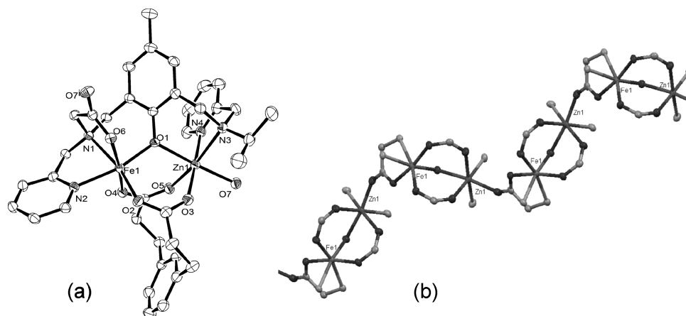
Figure 5. (a) ORTEP representation of the crystal structure of one monomer of [\text{Fe(III)Zn(II)(IPCPMP)(mpdp)}][\text{PF}_6] ( 6 ). (b) A Mercury plot of two repeating units in the polymeric network of 6 with only metals and atoms that are bridging and part of the polymeric backbone. All solvent and counterions have been omitted for clarity, and ellipsoids are drawn at 50% probability.
