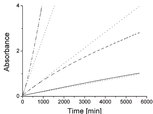
Figure 15. Kinetic traces of HPNP transesterification enhanced by [\text{Fe(III)M(II)(IPCPMP)(OAc)}_2(\text{CH}_3\text{OH})][\text{PF}_6] ( \text{M} = \text{Zn} ( 2 ) at pH 8.0 (—), \text{Co} ( 3 ) at pH 9.0 (---), and \text{Ni} ( 4 ) at pH 9.0 (···)). The dotted lines are linear fits to the initial parts (20–80 min) of the curves. Complex and substrate concentrations are 0.025 mM and 0.80 mM, respectively.
