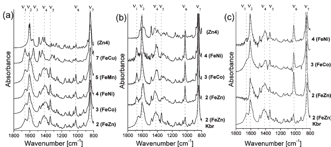
Figure 7. Fourier transform IR spectra of complexes [\text{Fe(III)M(II)(IPCPMP)(OAc)}_2(\text{CH}_3\text{OH})][\text{PF}_6] ( \text{M} = \text{Zn} (2), \text{Co} (3), \text{Ni} (4), \text{Mn} (5)), [\text{Fe(III)Cu(II)(IPCPMP)(OAc)}_2(\mu\text{-O})][\text{PF}_6] (7), and [\text{Zn}_2(\text{IPCPMP)(OAc)}_2][\text{PF}_6] (Zn4) in KBr (a). Solution FTIR of 2, 3, 4 and Zn4 40 mM in acetonitrile (b) and 2, 3, and 4 40 mM in \text{H}_2\text{O}/\text{MeCN} 1:1 v/v (c). The intensities have been adjusted using the strong absorption at 843\text{ cm}^{-1} for \text{PF}_6^- as internal standard. The spectra are numbered after their corresponding complexes. In the middle and bottom graphs the spectrum of 2 in KBr has been added as a reference.
