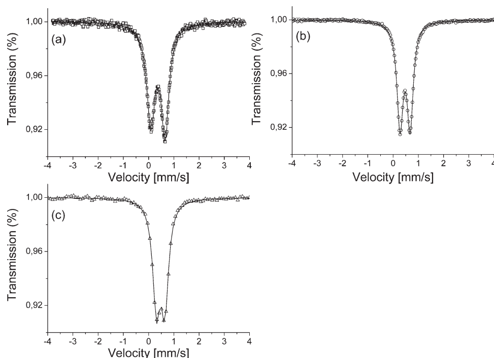
Figure 10. Mössbauer spectra at 80 K of [\text{Fe}(\text{III})(\text{H}_2\text{IPCPMP})(\text{Cl}_2)][\text{PF}_6] ( 1 ) (a), [\text{Fe}(\text{III})\text{Co}(\text{II})(\text{IPCPMP})(\text{OAc})_2(\text{CH}_3\text{OH})][\text{PF}_6] ( 3 ) (b), and [\text{Fe}(\text{III})\text{Mn}(\text{II})(\text{IPCPMP})(\text{OAc})_2(\text{CH}_3\text{OH})][\text{PF}_6] ( 5 ) (c) in the solid state.
