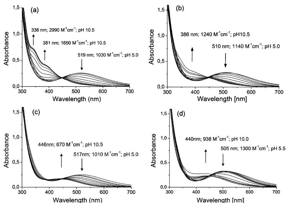
Figure 8. Dependence on pH of the spectra of [\text{Fe(III)M(II)(IPCPMP)(OAc)}_2(\text{CH}_3\text{OH})][\text{PF}_6] ( \text{M} = \text{Zn} (2), \text{Co} (3), \text{Ni} (4), \text{Mn} (5)). The arrows indicate the decrease and increase in intensity of specific bands when going from pH 5 to 10.5 in steps of 0.5.
