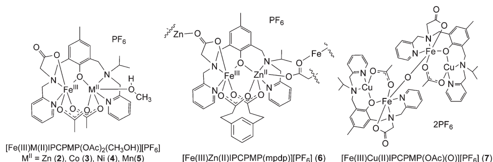
Chart 1. Schematic Depiction of the New Complexes Presented in This Work
