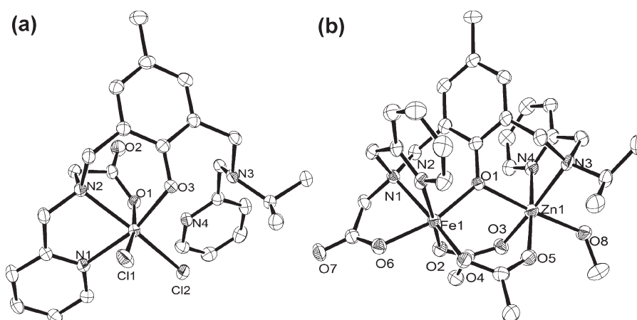
Figure 3. ORTEP 96 representations of [\text{Fe}(\text{III})(\text{H}_2\text{IPCPMP})(\text{Cl}_2)][\text{PF}_6] (1) (a) and [\text{Fe}(\text{III})\text{Zn}(\text{II})(\text{IPCPMP})(\text{OAc})_2(\text{CH}_3\text{OH})][\text{PF}_6] (2) (b) from ref 49.
