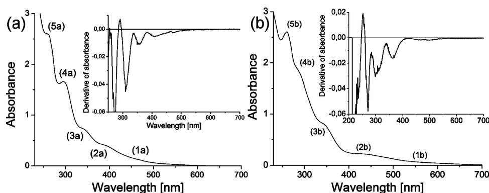
Figure 9. UV-vis spectrum of (a) [\text{Fe(III)Zn(II)(IPCPMP)(OAc)}_2(\text{CH}_3\text{OH})][\text{PF}_6] ( 2 ) at pH 10, 0.25 mM in acetonitrile/water 1:1, and (b) [\text{Fe(III)Cu(II)(IPCPMP)(OAc)}_2(\mu\text{-O})][\text{PF}_6] ( 7 ), 0.1 mM in acetonitrile. The inset displays the derivative of the absorbance vs the wavelength to more clearly display the shoulders present in the spectra.
