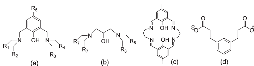
Figure 2. Schematic depiction of ligands that have been used to model active sites in PAPs. Type (a) includes ICIMP ( R_1 = R_4 = 1 -methylimidazole, R_2 = \text{CO}_2^- , R_3 = \text{iso-propyl} ; R_5 = \text{CH}_3 ) BPBPMP ( R_1 = R_2 = R_3 = 2 -pyridyl, R_4 = 2 -phenolate, R_5 = \text{CH}_3 ), BPMP ( R_1 = R_2 = R_3 = R_4 = 2 -pyridyl, R_5 = \text{CH}_3 ), BPBP ( R_1 = R_2 = R_3 = R_4 = 2 -pyridyl, R_5 = t -butyl), BHBPMP ( R_1 = R_2 = 2 -pyridyl, R_3 = R_4 = 2 -phenol, R_5 = \text{CH}_3 ), BPMOP ( R_1 = R_2 = R_3 = R_4 = 2 -pyridyl, R_5 = \text{methoxy} ). Type (b) includes tdmppo ( R_7 = R_8 = 4,5 -dimethylbenzimidazolyl); thebpo ( R_7 = R_8 = (2 -hydroxyethyl)benzimidazolyl); bdmppo ( R_7 = (4,5 -dimethyl)benzimidazolyl, R_8 = 2 -pyridyl). (c) Macrocyclic bis-phenolato ligand. The present study involves type (a) IPCPMP ( R_1 = R_4 = 2 -pyridyl, R_2 = \text{CO}_2^- , R_3 = \text{iso-propyl} , R_5 = \text{CH}_3 ) (d) 1,3- meta -phenylenedipropionate (mpdp).
