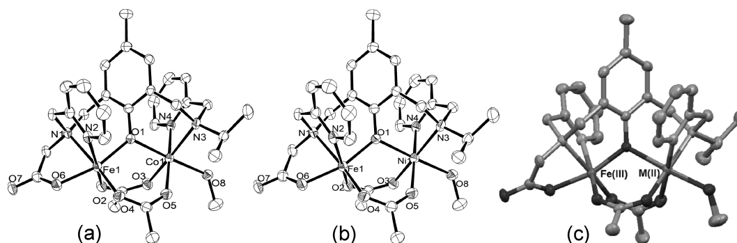
Figure 4. ORTEP representations of the crystal structures of [\text{Fe}(\text{III})\text{Co}(\text{II})(\text{IPCPMP})(\text{OAc})_2(\text{CH}_3\text{OH})][\text{PF}_6] (3) (a) and [\text{Fe}(\text{III})\text{Ni}(\text{II})(\text{IPCPMP})(\text{OAc})_2(\text{CH}_3\text{OH})][\text{PF}_6] (4) (b) along with a Mercury 97 overlay structure of complexes 2, 3, and 4 (c), where \text{M}(\text{II}) = \text{Zn}(\text{II}), \text{Co}(\text{II}), or \text{Ni}(\text{II}) , respectively. All solvent molecules and counterions have been omitted for clarity, and the ellipsoids are drawn at 50% probability. The ( R,R ) enantiomers are shown in (a) and (b) while in (c) only the ( S,S ) enantiomers were overlaid.
