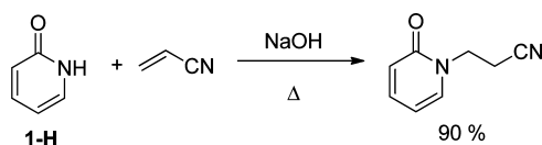
Scheme 6. Selective N -Alkylation of 2-Pyridone Anion with Acrylonitrile 26
