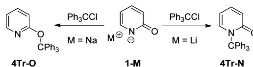
Scheme 8. Selective O - and N -Tritylation of Pyridone Salts in Acetonitrile 27
