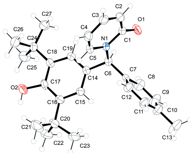
Figure 3. Crystal structure of the reaction product 4l-N obtained from 1a-K and 2l (50% probability ellipsoids).
