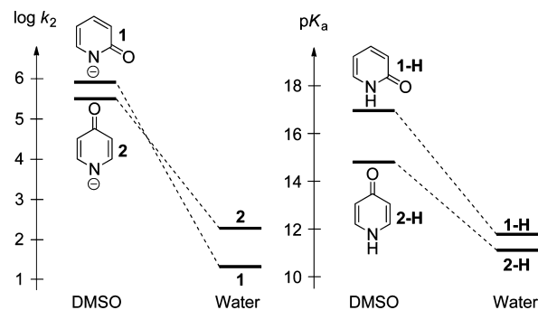
Scheme 2. Solvent Dependence of the Rate Constant of the Reactions of 1-K and 2-K with 3h at 20 °C and the Corresponding \text{p}K_{\text{a}} Values ( \text{p}K_{\text{a}} from ref 16)
