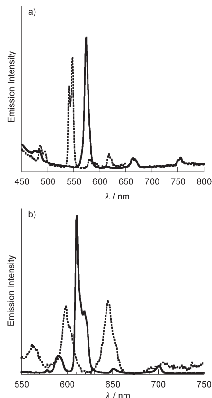
Figure 6. The corrected emission spectra of the visible emitting complexes in acetonitrile, \lambda_{\text{exc}} = 270 nm. Top: [Tb(F 20 tpip) 3 ] (-----) and [Dy(F 20 tpip) 3 ] (—) displaying Tb III -based 5 D 4 → 7 F J ( J = 3, 4, 5, 6) and Dy III -based 4 F 9/2 → 6 H J ( J = 15/2, 13/2, 11/2, 9/2) transitions respectively. Bottom: [Sm(F 20 tpip) 3 ] (-----) and [Eu(F 20 tpip) 3 ] (—) in acetonitrile, displaying Sm III -based 4 G 5/2 → 6 H J ( J = 5/2, 7/2, 9/2 and 11/2) and Eu III -based 5 D 0 → 7 F J ( J = 0, 1, 2, 3, 4) transitions, respectively.
