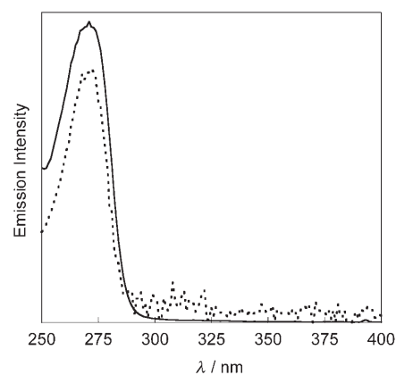
Figure 9. Excitation (solid line) and absorption (dotted line) spectra of [\text{Eu}(\text{F}_{20}\text{tpip})_3] in acetonitrile, \lambda_{\text{em}} = 610 nm.
