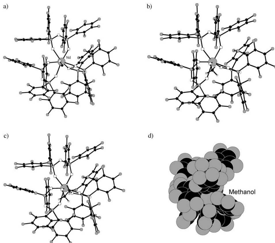
Figure 2. The complexes of a) 1 , b) 3a , c) 3b and d) a space filling representation of 1 with the methanol molecule omitted to show the slot it occupies
