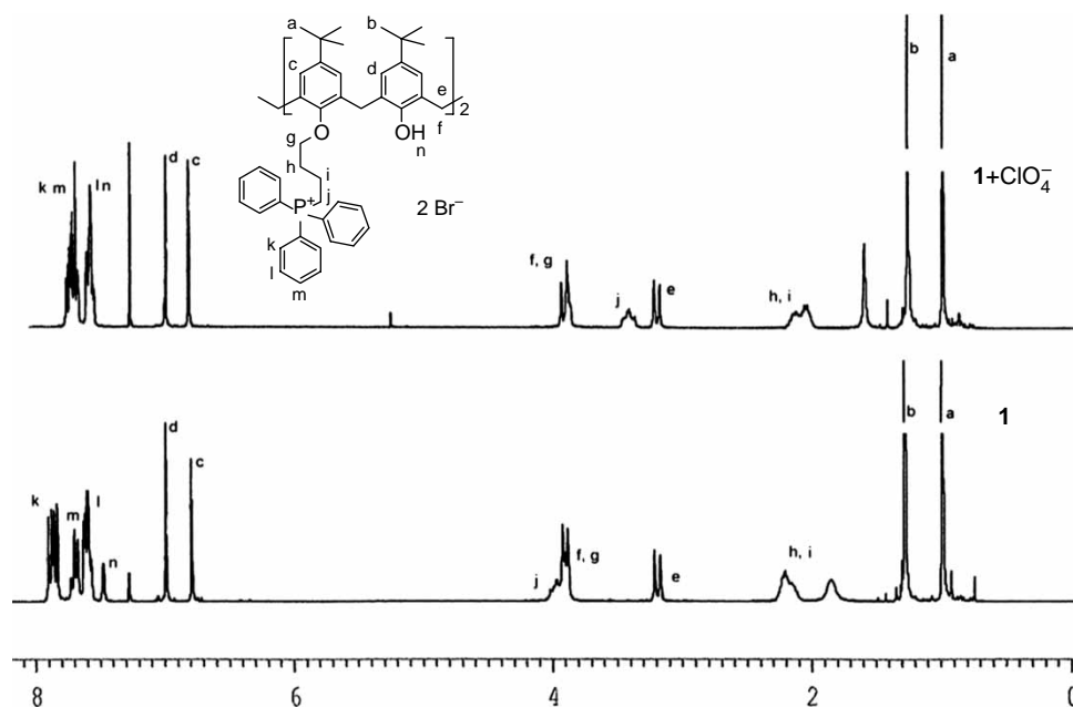
Figure 2. ^1\text{H} NMR spectra of ligand 1 alone and in the presence of \text{ClO}_4^- in \text{CDCl}_3 .
