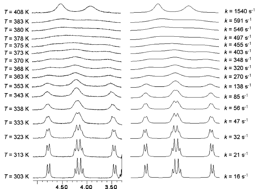
FIGURE 2. Partial (protons at C2 carbon) VT-NMR spectra of 1a (5 mM, DMSO- d_6 , 300 MHz): experimental (left) and simulated (right). Values of temperature ( T , K) and interconversion rate ( k , s^{-1} ) are also given for every trace. Simulated spectra were obtained with the gNMR program. 23
