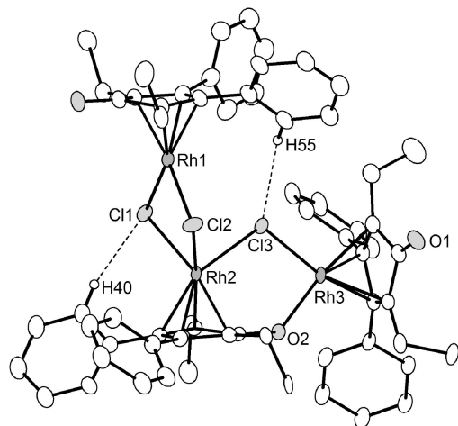
Figure 1. Molecular structure of complex 4 in the crystal. The crystallized solvent molecule (CH 2 Cl 2 ) and the hydrogen atoms, except those involved in secondary interactions, are not shown for clarity. The thermal ellipsoids are set at 50% probability.
